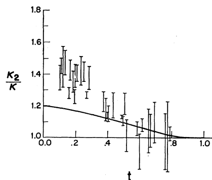
FIG. 8. Values of \kappa_2/\kappa which would lead to agreement between theory and experiment for S_e .
