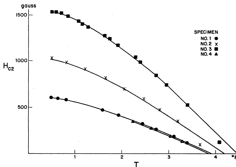
FIG. 4. Variation of the upper critical field with temperature for specimens 1-4.
