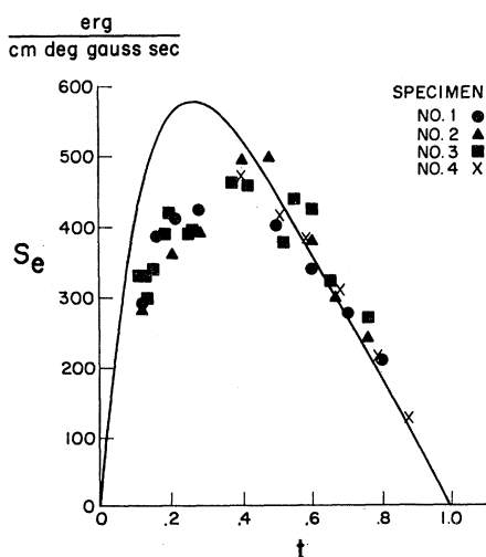
FIG. 7. Corrected ratios S_e = (dK_e/dH)_{H_{e2}} \times 1.16(2\kappa_2^2 - 1) .
