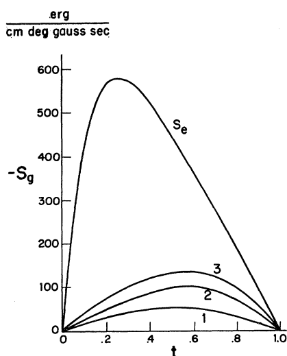
FIG. 6. Calculated ratios S_g = (dK_g/dH)_{H_{e2}} \times 1.16(2\kappa_2^2 - 1) together with the theoretical curve for S_e .
