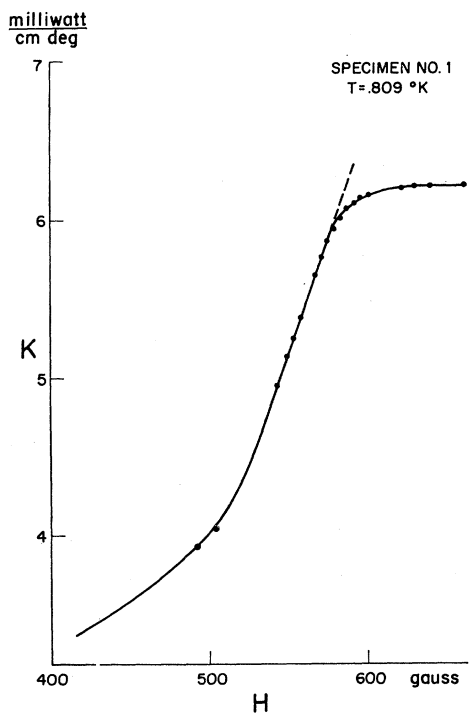
FIG. 2. Example of a curve of thermal conductivity against field.
