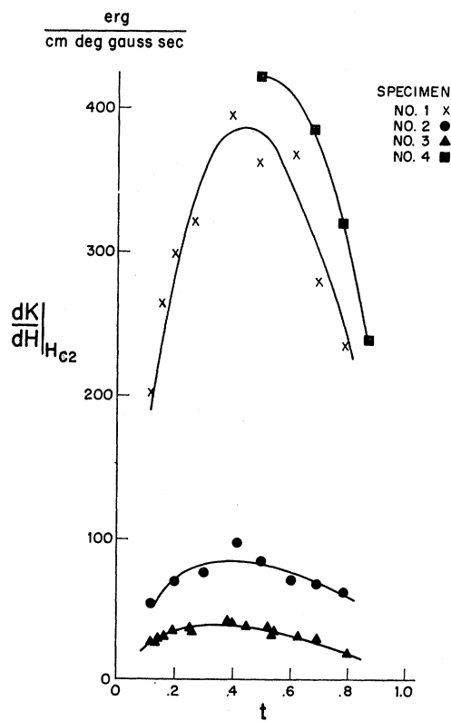
FIG. 3. Measured slopes (dK/dH)_{H_{c2}} as a function of reduced temperature.
