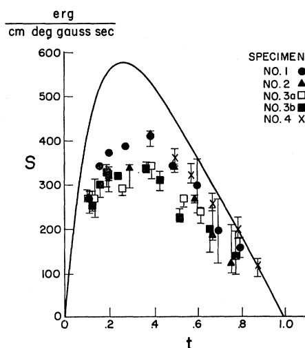
FIG. 5. Measured ratios S = (dK/dH)_{H_{c2}} \times 1.16(2\kappa_2^2 - 1) .
