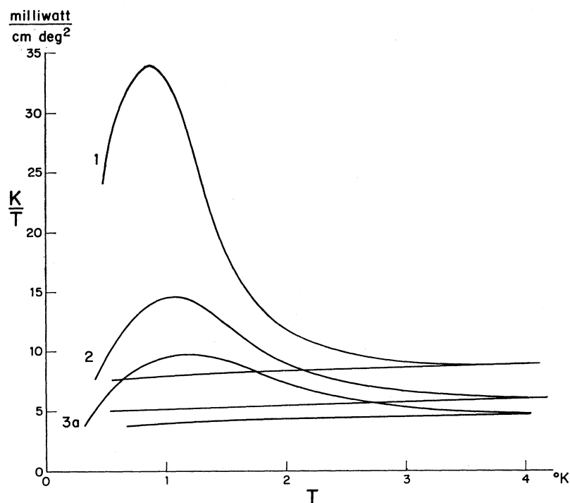
FIG. 1. Thermal conductivity of specimens 1, 2, and 3a plotted as K/T against T . In each case the upper curve represents the results in the superconducting state and the lower curve the results in the normal state.
